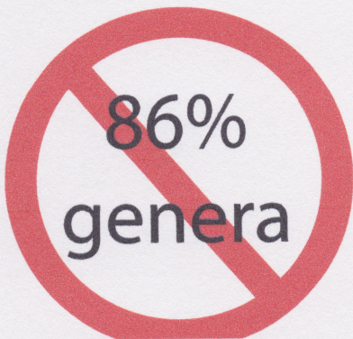
Permo-Triassic Mass Extinction
