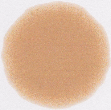
Formation of Planet Earth
